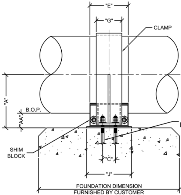
ELEVATION AT PIPE SUPPORT
