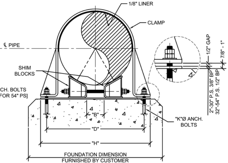
SECTION THRU PIPE AT SUPPORT
