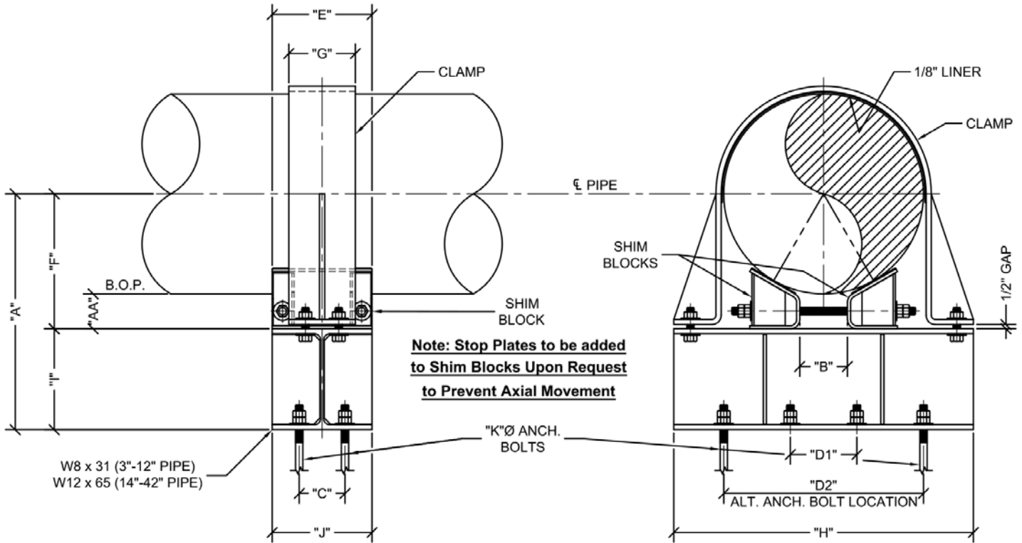
ELEVATION AT PIPE SUPPORT
